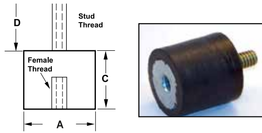
MALE STUD - FEMALE SOCKET ISOLATORS
